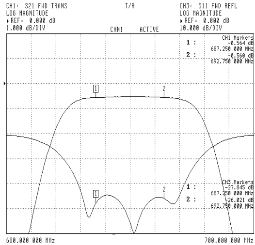
Input Insertion Loss and Return Loss
